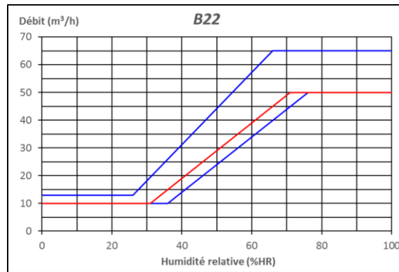
Figure 27– B22 (5-45 m3/h, 43-83%HR)
