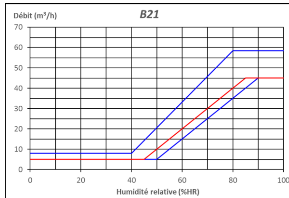
Figure 26 – B21 (5-45 m3/h, 45-85%HR)
