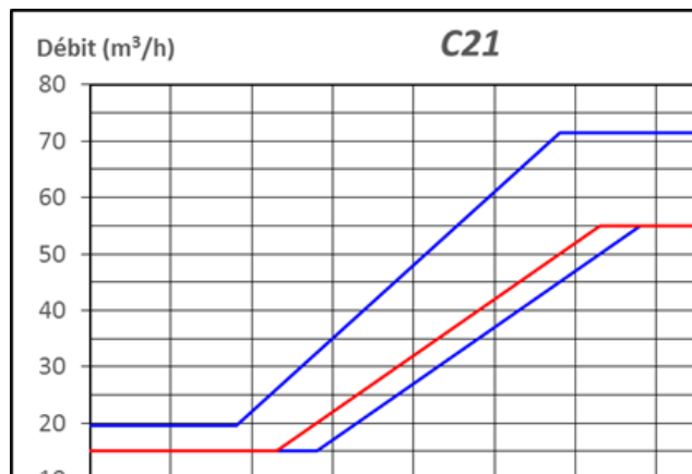
Figure 23 – C21 (15-55/135 m³/h, 23-63%HR)
