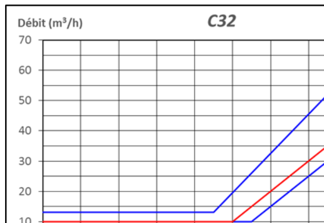
Figure 24 – C32 (10-50/90 m³/h, 50-90%HR)
