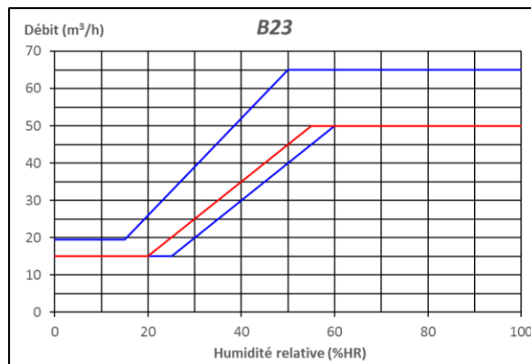
Figure 28 – B23 (15-50 m3/h, 20-55%HR)
