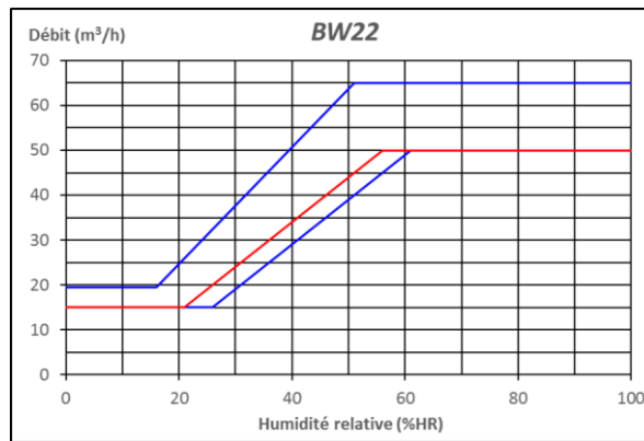
Figure 30 – BW22 (15-50/50 m³/h, 21-56%HR)
